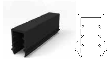
"U" SHAPE GASKET FOR 11.52mm GLASS JOINT DU GUIDAGE POUR VERRE 11.52mm
