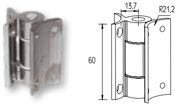
HINGE FOR F50-100 COLUMN CHARNIERE DE POTEAU F50-100
