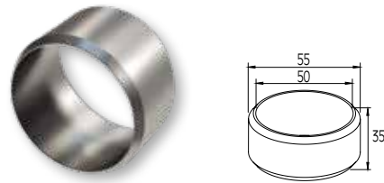
CONNECTOR FOR HANDRAIL Ø50 JONCTION DE MAIN COURANTE Ø50
