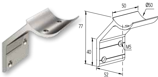
FIXED WALL SUPPORT FOR F50-200 HANDRAIL FIXATION MURALE DE MAIN COURANTE F50-200
