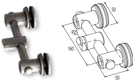
SINGLE GLASS SUPPORT 8-10mm FOR Ø50 COLUMN DOUBLE FIXATION DE VERRE 8-10mm DE POTEAU Ø50
