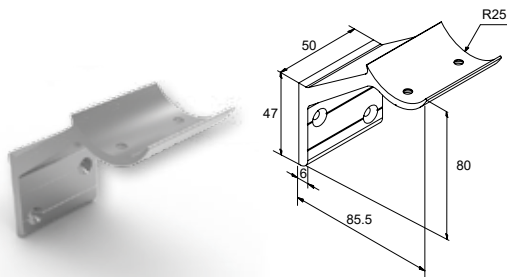
FIXED WALL SUPPORT FOR F50-200 HANDRAIL FIXATION MURALE DE MAIN COURANTE F50-200
