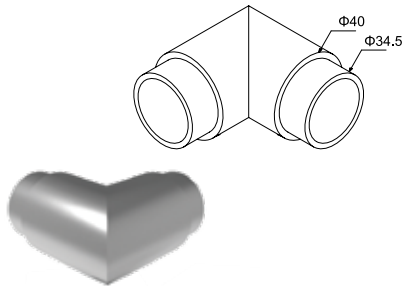
CODE 4277 CONNECTOR 90° FOR HANDRAIL Ø40 JONCTION 90° DE MAIN COURANTE Ø40 PRICE / PRIX 6,95 €/pc
