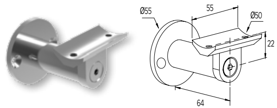
WALL SUPPORT FOR F50-200 HANDRAIL FIXATION MURALE DE MAIN COURANTE F50-200
