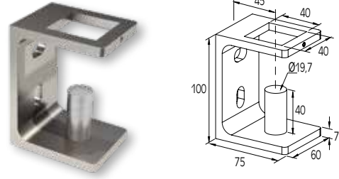
EXTERNAL SUPPORT FOR F50-102 COLUMN FIXATION MURALE DE POTEAU F50-102
