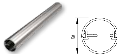
PERFORATED GUIDE Ø26 GUIDAGE PERFORE Ø26
