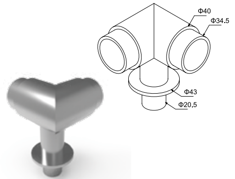
CODE 4262 CONNECTOR 90° FOR HANDRAIL Ø40 JONCTION 90° DE MAIN COURANTE Ø40 PRICE / PRIX 11,90 €/pc
