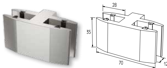
EXTERNAL DOUBLE GLASS SUPPORT 8-10mm FOR F50-102 COLUMN DOUBLE FIXATION EXTERIEURE DE VERRE 8-10mm DE POTEAU F50-102
