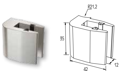
SINGLE GLASS SUPPORT 8-10mm FOR F50-103 COLUMN SINGLE FIXATION EXTERIEURE DE VERRE 8-10mm DE POTEAU F50-103
