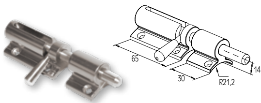
BOLT FOR F50-100 COLUMN VERROU DE POTEAU F50-101
