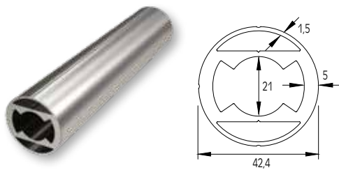
SUPPORT COLUMN Ø42 (HEAVY-DUTY) POTEAU Ø42 ROBUSTE
