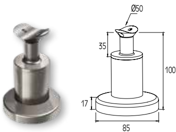
SUPPORT FOR F50-200 HANDRAIL FIXATION DE MAIN COURANTE F50-200
