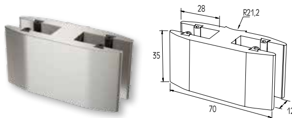
DOUBLE GLASS SUPPORT 8-10mm FOR F50-103 COLUMN DOUBLE FIXATION EXTERIEURE DE VERRE 8-10mm DE POTEAU F50-103
