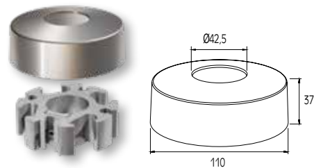
SUPPORT FOOT FOR Ø42 COLUMN SABOT DE POTEAU Ø42
