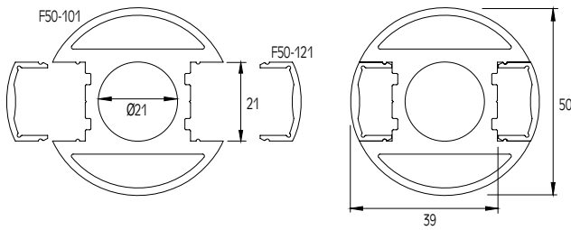
COVER FOR F50-101 COLUMN CAPUCHON DE POTEAU F50-101
