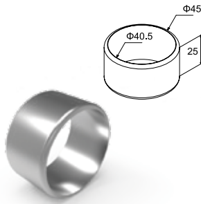
CODE 4260 CONNECTOR FOR HANDRAIL Ø40 JONCTION DE MAIN COURANTE Ø40 PRICE / PRIX 3,20 €/pc
