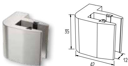
EXTERNAL SINGLE GLASS SUPPORT 8-10mm FOR F50-102 COLUMN SINGLE FIXATION EXTERIEURE DE VERRE 8-10mm DE POTEAU F50-102
