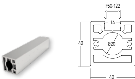
SUPPORT COLUMN 40x40 POTEAU 40x40
