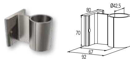
EXTERNAL SUPPORT FOR Ø42 COLUMN FIXATION EXTERIEURE DE POTEAU Ø42
