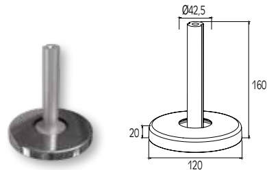
SUPPORT FOOT FOR Ø42 COLUMN SABOT DE POTEAU Ø42
