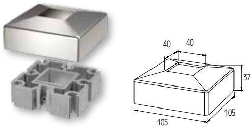
SUPPORT FOOT FOR 40x40 COLUMN SABOT DE POTEAU 40x40
