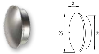
END CAP FOR F50-304 PROFILE EMBOUT DE PROFIL F50-304
