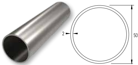
HANDRAIL Ø50 MAIN COURANTE Ø50
