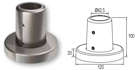
HEAVY DUTY SUPPORT FOOT FOR Ø42 COLUMN SABOT DE POTEAU Ø42 ROBUSTE
