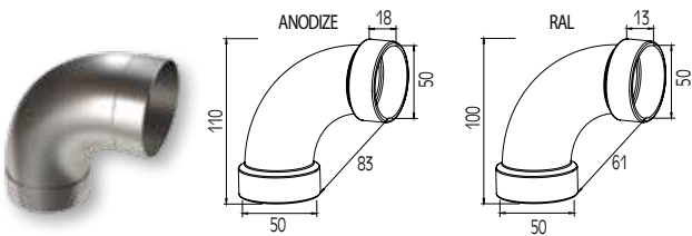
CONNECTOR FOR HANDRAIL Ø50 JONCTION 90° DE MAIN COURANTE Ø50
