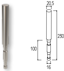
INFLOOR SUPPORT FOR Ø42 COLUMN FIXATION ENCASTRE DE POTEAU Ø42
