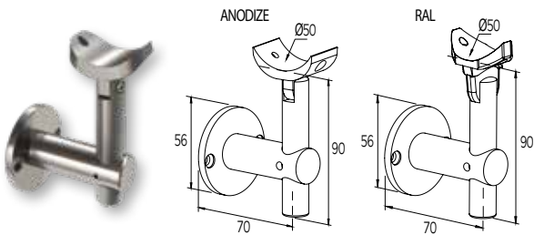
SUPPORT FOR F50-200 HANDRAIL FIXATION MURALE DE MAIN COURANTE F50-200
