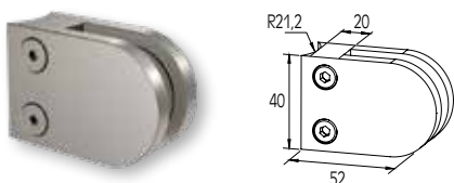
INOX GLASS SUPPORT 6-8mm INOX FIXATION DE VERRE 6-8mm INOX
