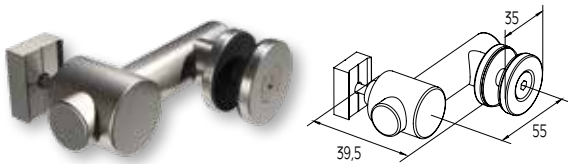
SINGLE GLASS SUPPORT 8-10mm FOR BLADE COLUMN FIXATION DE VERRE 8-10mm DE POTEAU BLADE
