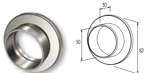
WALL COVER FOR HANDRAIL Ø50 WITH CAP CACHE DU MUR DE MAIN COURANTE Ø50(+CAPUCHON)
