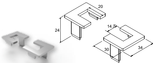
END CAP FOR F50-319 GUIDE (PERFORATED) EMBOUT OUVERTE DE GUIDAGE F50-319
