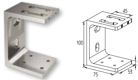
EXTERNAL SUPPORT FOR BLADE COLUMN FIXATION EXTERIEURE DE POTEAU BLADE
