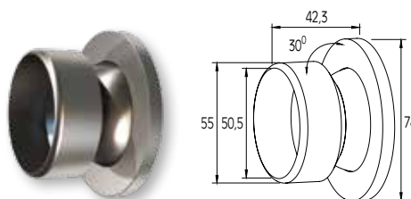
WALL COVER FOR HANDRAIL Ø50 WITH CAP CACHE DU MUR DE MAIN COURANTE Ø50 (+CAPUCHON)
