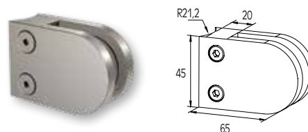
GLASS SUPPORT 8-10mm INOX FIXATION DE VERRE 8-10mm INOX
