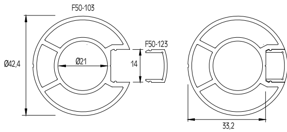
COVER FOR F50-103 COLUMN CAPUCHON DE POTEAU F50-103
