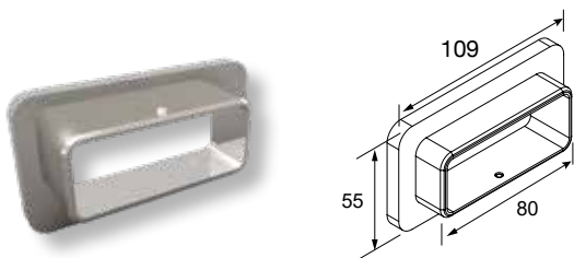
WALL COVER FOR F50-201/203 HANDRAIL (WITH CAP) CACHE DU MUR DE MAIN COURANTE F50-201/203 (+CAPUCHON)
