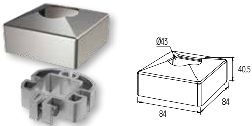
SUPPORT FOOT FOR Ø42 COLUMN SABOT DE POTEAU Ø42
