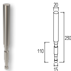
INFLOOR SUPPORT FOR F50-102 COLUMN FIXATION ENCASTRE DE POTEAU F50-102
