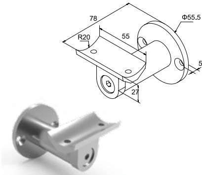
CODE 4135 WALL SUPPORT FOR Ø40 HANDRAIL FIXATION MURALE DE MAIN COURANTE Ø40 PRICE / PRIX 6,05 €/pc
