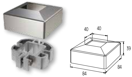
SUPPORT FOOT FOR 40x40 COLUMN SABOT DE POTEAU 40x40
