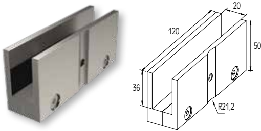
DOUBLE GLASS SUPPORT 19-22mm FIXATION DOUBLE DE VERRE 19-22mm
