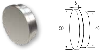
END CAP FOR F50-200 HANDRAIL (FLAT) EMBOUT DE MAIN COURANTE F50-200 (PLAT)
