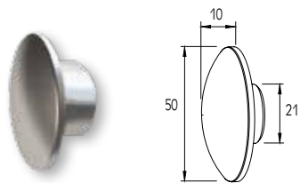
END CAP FOR F50-101 COLUMN EMBOUT DE POTEAU F50-101
