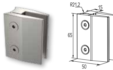
GLASS SUPPORT 8-10mm FIXATION DE VERRE 8-10mm
