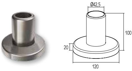
EXTERNAL SUPPORT FOOT FOR Ø42 COLUMN SABOT EXTERIEUR DE POTEAU Ø42
