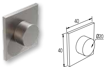
END CAP FOR F50-102 COLUMN EMBOUT DE POTEAU F50-102
