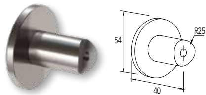
EXTERNAL SUPPORT FOR F50-101 COLUMN FIXATION EXTERIEURE DE POTEAU F50-101
