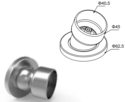
CODE 4521 WALL COVER FOR HANDRAIL Ø40 WITH CAP CACHE DU MUR DE MAIN COURANTE Ø40 (+CAPUCHON) PRICE / PRIX 10,10 €/pc
