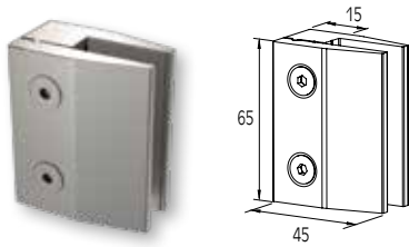
SINGLE GLASS SUPPORT 8-10mm FOR F50-102/106 COLUMN SINGLE FIXATION EXTERIEURE DE VERRE 8-10mm DE POTEAU F50-102/106
