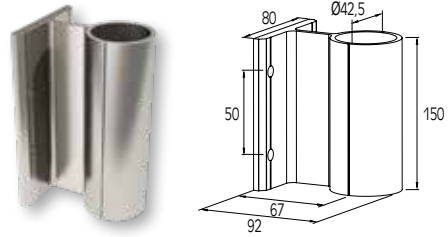
EXTERNAL WALL SUPPORT FOR COLUMN Ø42 FIXATION MURALE EXTERIEURE DE POTEAU Ø42
