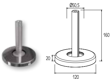
SUPPORT FOOT FOR Ø50 COLUMN SABOT DE POTEAU Ø50
