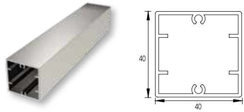
SUPPORT COLUMN 40x40 POTEAU 40x40
