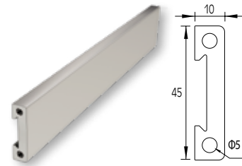
BLADE COLUMN POTEAU BLADE
