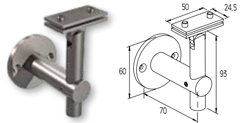
F50-201 RAILTOP WALL SUPPORT F50-201 RAILTOP WALL SUPPORT
