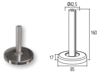
SUPPORT FOOT FOR Ø42 COLUMN SABOT DE POTEAU Ø42
