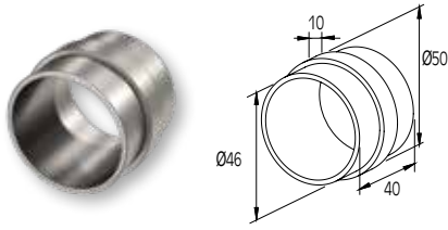
CONNECTOR FOR HANDRAIL Ø50 (INTERNAL) JONCTION DE MAIN COURANTE F50 (INTERNE)
