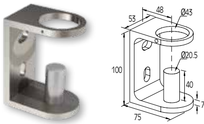
EXTERNAL SUPPORT FOR F50-100/103 COLUMN FIXATION MURALE DE POTEAU F50-100/103
