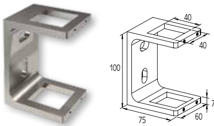
EXTERNAL SUPPORT FOR 40x40 COLUMN FIXATION EXTERIEURE DE POTEAU 40x40
