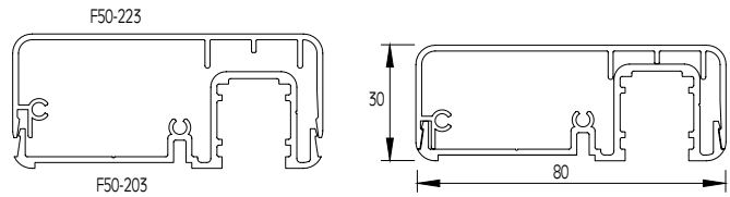
COVER FOR DIVIDABLE HANDRAIL F50-203 CAPUCHON DE MAIN COURANTE F50-203 (DIVISE)
