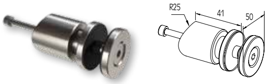
SINGLE GLASS SUPPORT 8-10mm FOR F50-101 COLUMN FIXATION DE VERRE 8-10mm DE POTEAU F50-101
