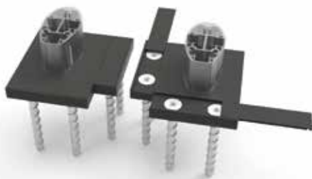
CORNER SUPPORT FOOT FOR COLUMN FSN-102 SABOT DE COIN DE POTEAU FSN-102
