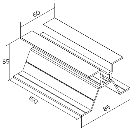
E5302-071 (150mm) Landscape Panels' Array ROOF STEP= 250mm
