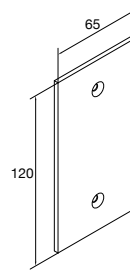
272-268 End Cover for 2050-102
