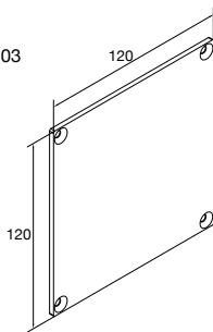
2050-002 Connector for 2050-102 & 2050-103 (All Combinations)
