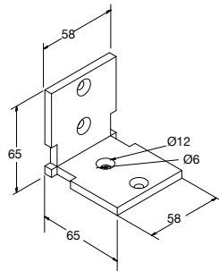
272-263 / 272-276 Base profile for rotation louver 2050-602 (3m)
