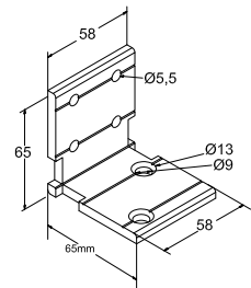
2050-012 Support for Column
