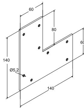
2050-022 Connector for Column
