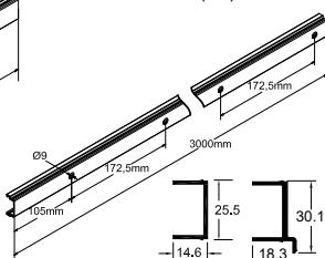
272-263 / 272-276 Base profile for rotation louver 2050-602 (3m)
