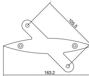
2050-052 Base profile for rotation louver 2050-611 (3m)
