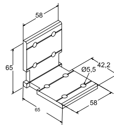
2050-022 Connector for Column
