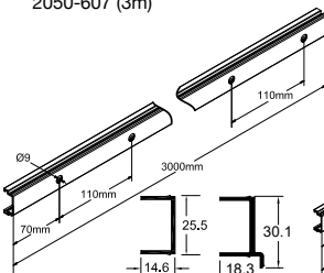
272-262 / 272-275 Base profile for rotation louver 2050-607 (3m)
