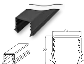
"U" shaped gasket / Joint Code F85-407 (10.10.4) for glass / pour verre 10 mm+4PVB+10 mm
