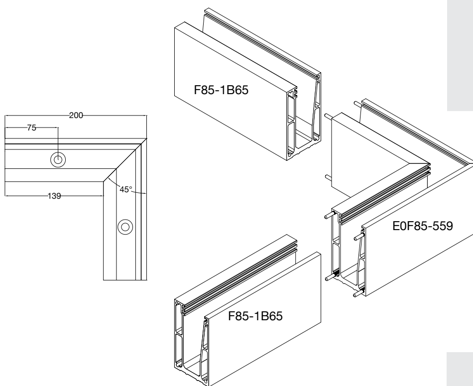
External Balcony Connectors
